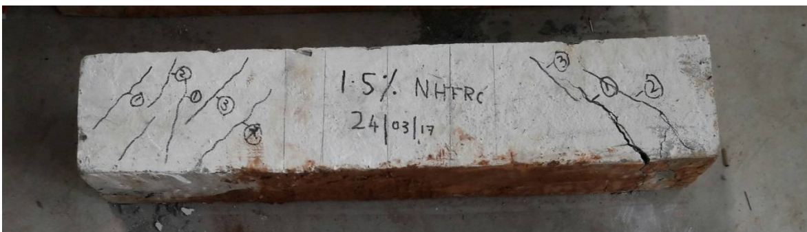
Figure4. Crack pattern for 1.5% NHFRC & 3% NS beam
