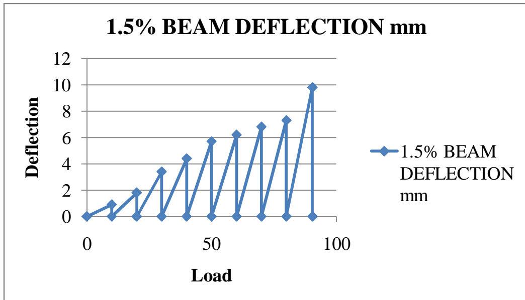
Graph1. Cycle VS Load at mid-span for 1.5% NS and 3% NHFRC
