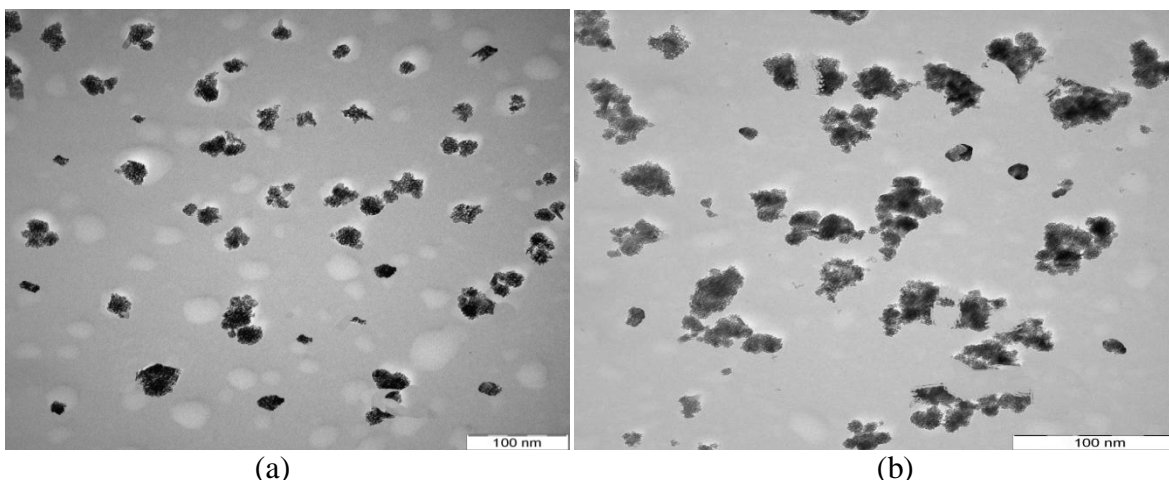
Figure 1: shows the TEM of (a) 30 nm Cr suspended in water for volume fraction 0.8% (b) 75 nm suspended on EG for volume fraction 0.8%.
