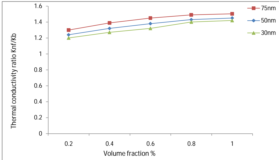
Figure 5: Depicting heat conductivity ratio of different size Cr nanoparticles with different size suspended in ethylene glycol for different volume fraction.
