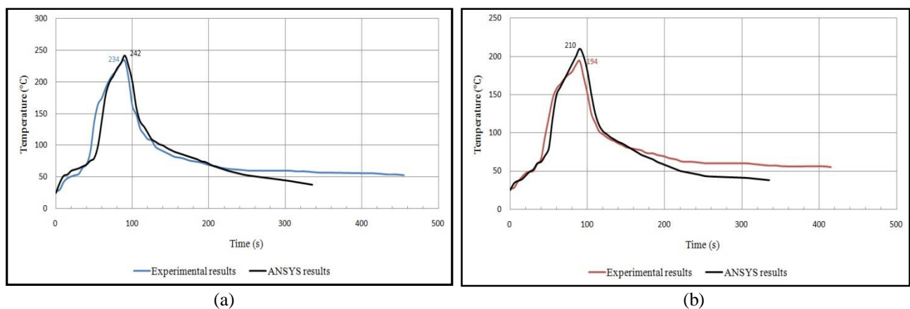
Figure 11: Comparison of the experimental and ANSYS model results obtained at different tested regions during FSSW using the triangular tool pin profile, (a) at the center of weld nugget (T1 location), (b) at a distance of 7mm from the center of the spot (T2 location)
