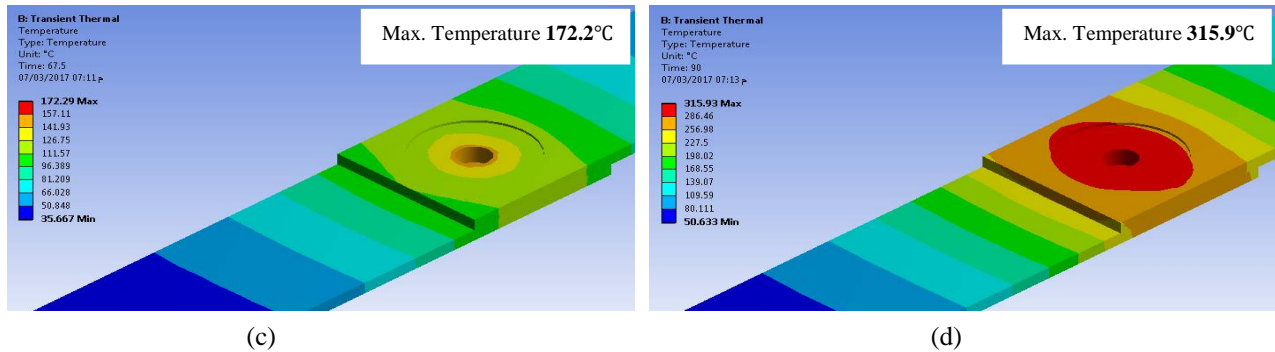
Figure 8: Isometric view of temperature distribution for different welding times in FSSW joint welded by the cylindrical tool pin profile, (a) 22.5sec, (b) 45sec, (c) 67.5sec, and (d) 90 sec
