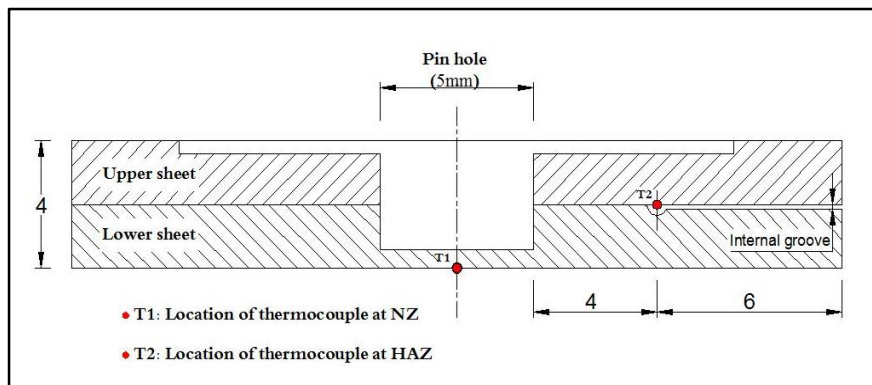
Figure 3: A schematic cross-section shows thermocouples sites
