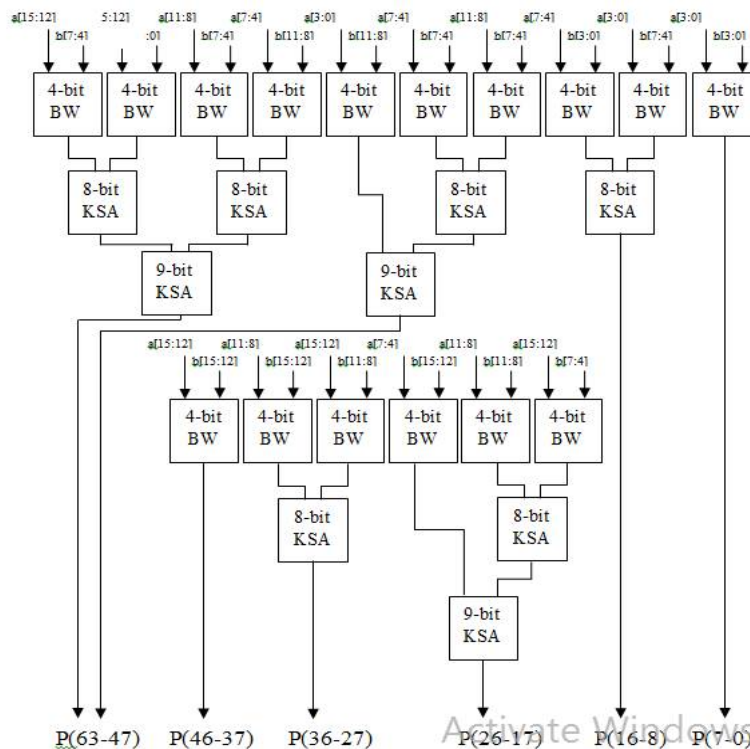
Figure 6: Linear Convolution based on Baugh multiplier and Kogge Stone adder
