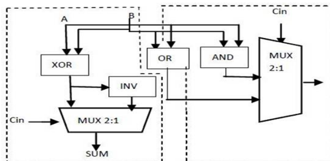
Figure 5: Block Diagram of CBL
