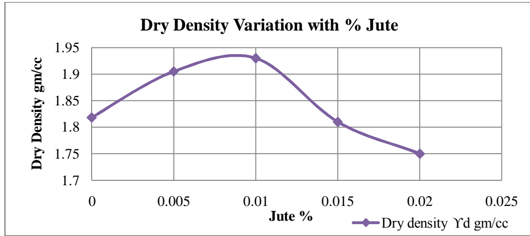
Figure 5: Dry Density/v/s Jute % Curve
