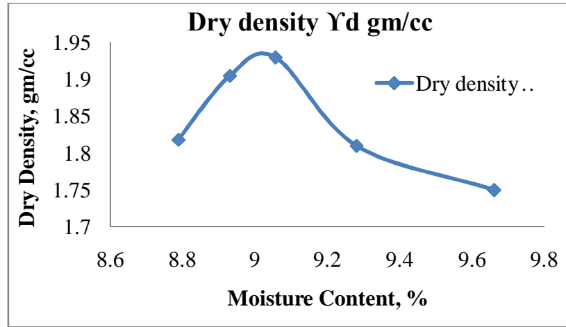
Figure 3: Dry Density v/s Moisture Content Curve
