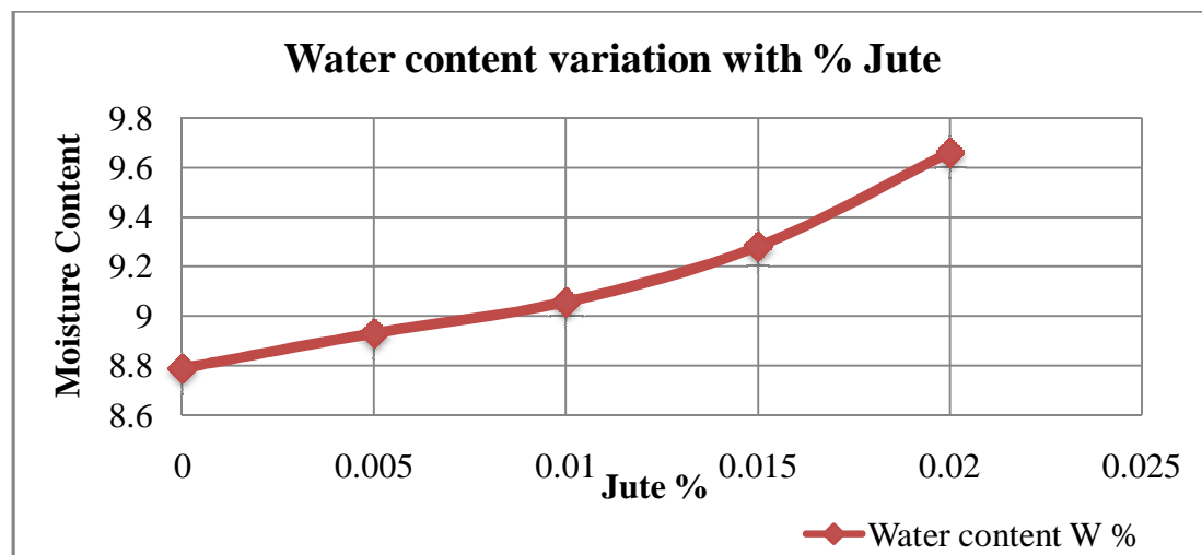
Figure 4: Moisture Content v/s Jute % Curve
