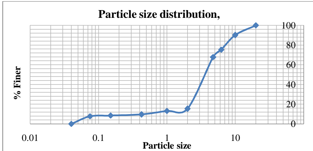
Figure 2: Particle Size Distribution Curve
