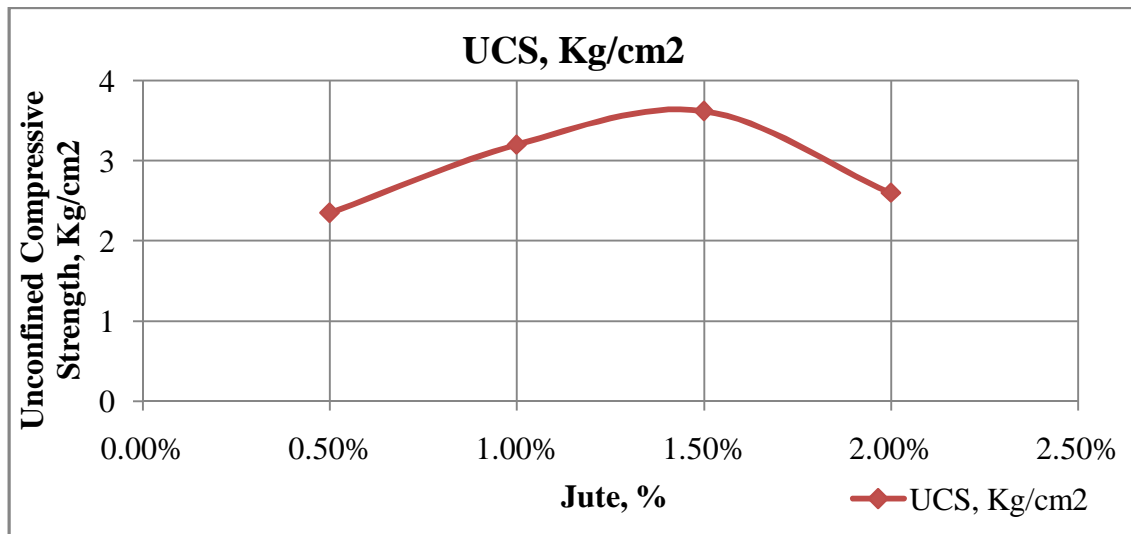
Figure 6: Unconfined Compressive Strength
