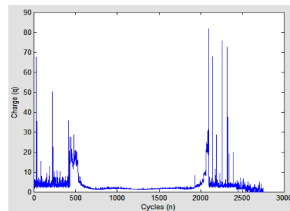
Fig.9 (e) Kurtosis plot (n-q) of corona discharge
