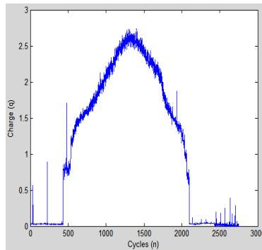
Fig.9 (b) Standard deviation (n-q) of corona discharge
