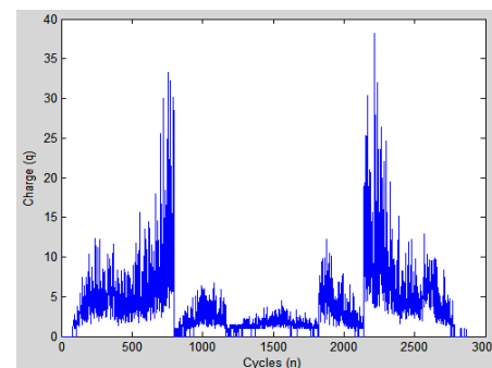
Fig.12 (e) Kurtosis plot (n-q) of data3
