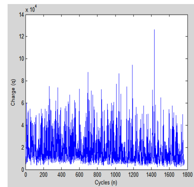
Fig.8 (c) Variance plot (n-q) of surface discharge
