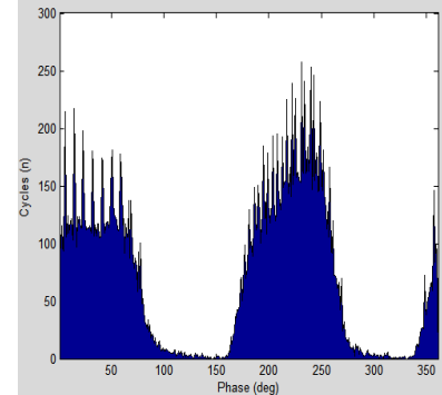
Fig.6(c). Phase plot ( \phi -n) of data3
