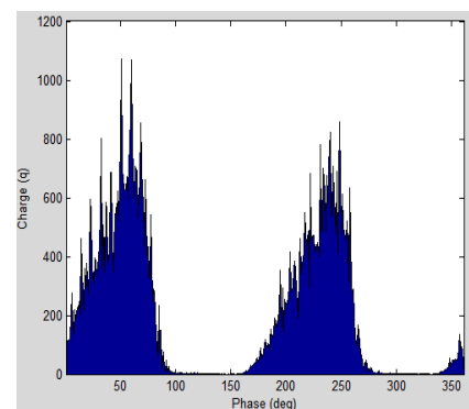
Fig.4 (c) Phase plot ( \phi -q) of data3
