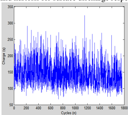
Fig.8 (a) Mean plot (n-q) of surface discharge
