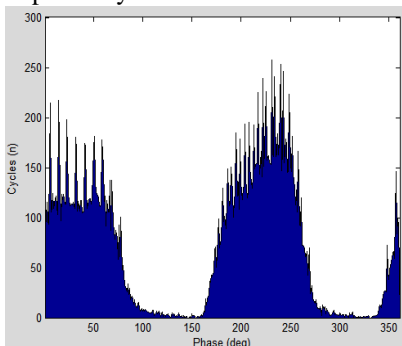
Fig.5(a).Phase plot (\varphi-n) of void discharge
