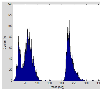
Fig.5(b).Phase plot (\varphi-n) of surface discharge
