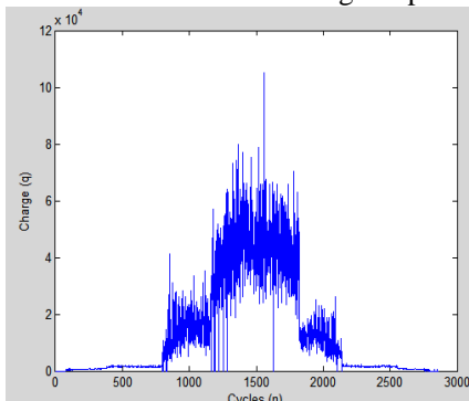
Fig.7(a). Mean plot (n-q) of void discharge
