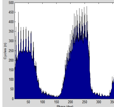
Fig.6(b). Phase plot ( \phi -n) of data2
