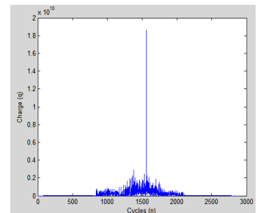
Fig.12 (c) Variance plot (n-q) of data3
