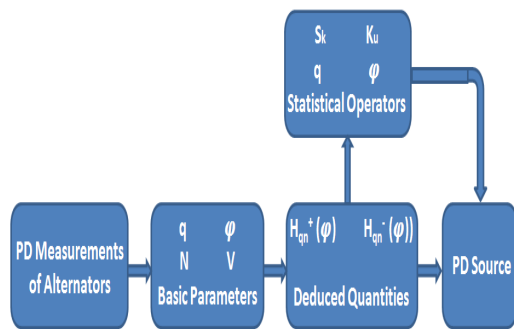
Fig.1 (a) Block diagram of discharge analysis for (\varphi-q)
