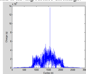
Fig.12 (b) Standard deviation plot (n-q) of data3
