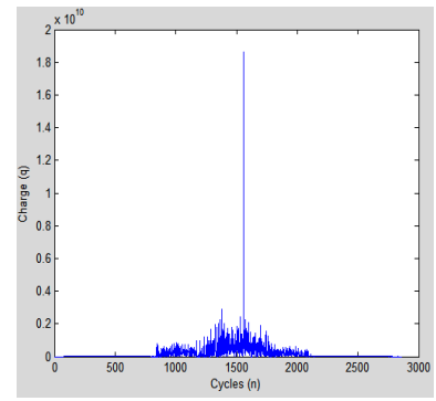
Fig.7(c). Variance plot (n-q) of void discharge
