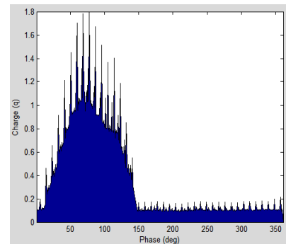
Fig.3(c). Phase plot ( \phi -q) of corona discharge
