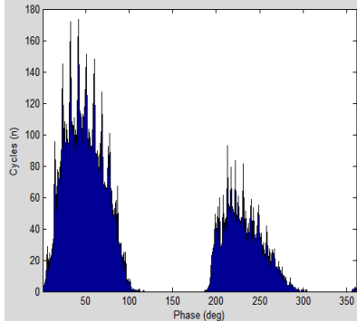
Fig.6(a). Phase plot ( \phi -n) of data1
