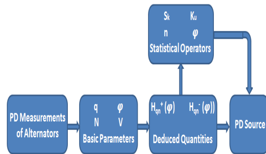
Fig.1 (a) Block diagram of discharge analysis for (\varphi-n)
