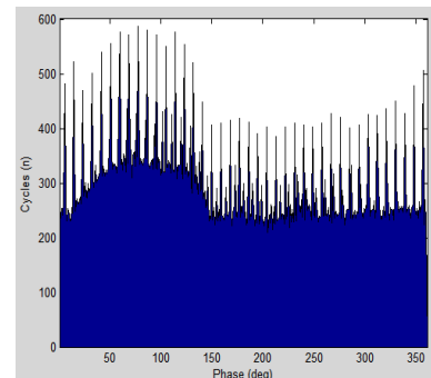
Fig.5(c).Phase plot (\varphi-n) of corona discharge
