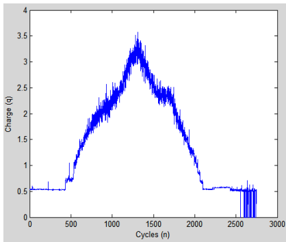
Fig.9 (a) Mean plot (n-q) of corona discharge
