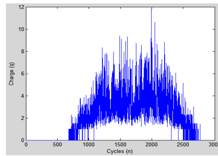
Fig.10 (e) Kurtosis plot (n-q) of data1
