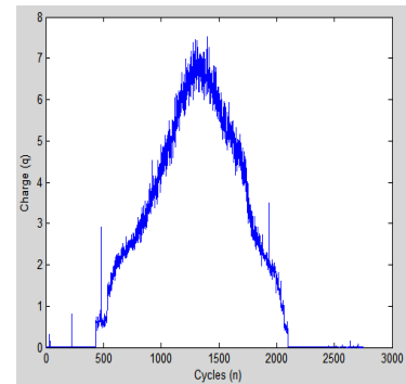
Fig.9 (c) Variance plot (n-q) of corona discharge
