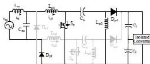
Fig. 2 Operation of PFC converter when the input voltage is positive
