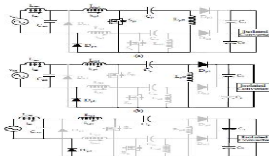
Fig. 3 Operating modes of bridgeless PFC converter when the input voltage is positive
