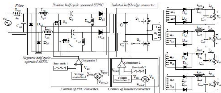
Fig.1 Schematic diagram of the PFC converter based SMPS
