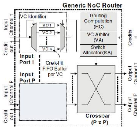
Figure 2. Generic NoC router architecture.
