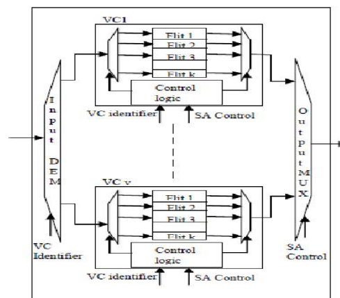
Figure 3. Buffer architecture for Generic NoC router.
