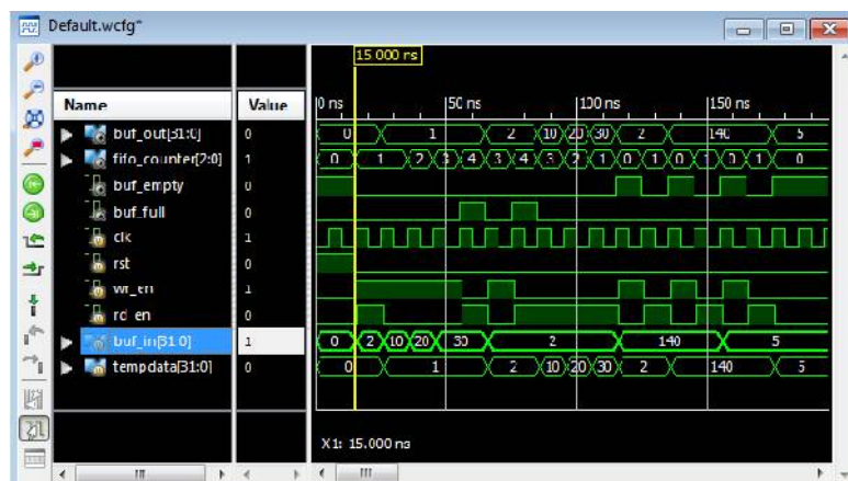
Figure 4. Simulation result for FIFO Buffer.
