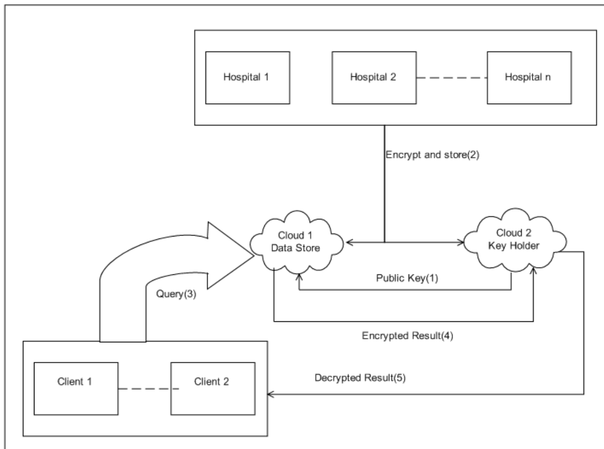
Fig 1: System Architecture
