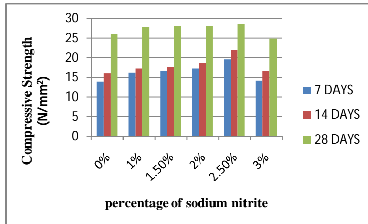
Fig: 4 Compressive strength results for sodium nitrite
