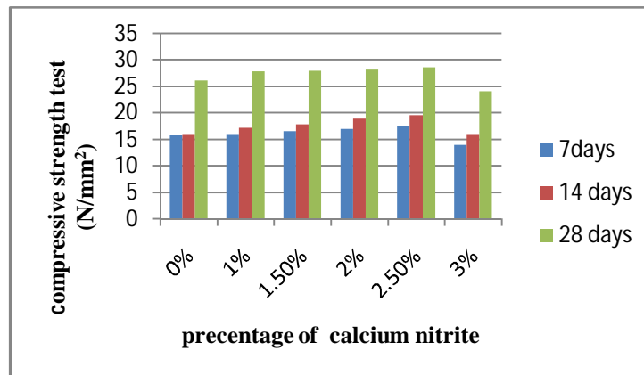
Fig: 5 compressive strength results for calcium nitrite
