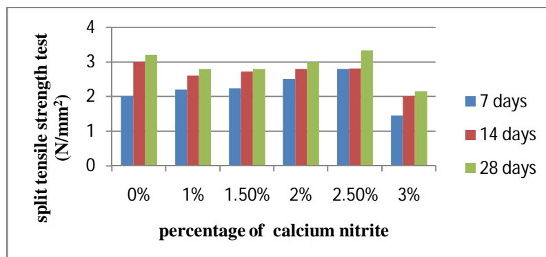
Fig: 8 split tensile strength results for calcium nitrite
