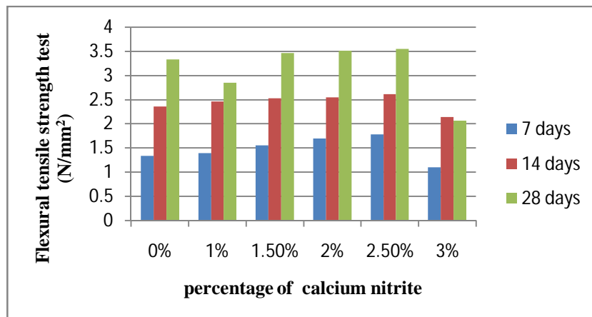
Fig: 10 Flexural strength results for calcium nitrite
