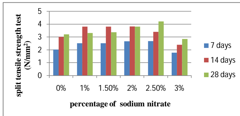
Fig: 7 split tensile strength results for sodium nitrite
