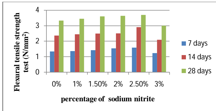
Fig: 9 Flexural strength results for sodium nitrite
