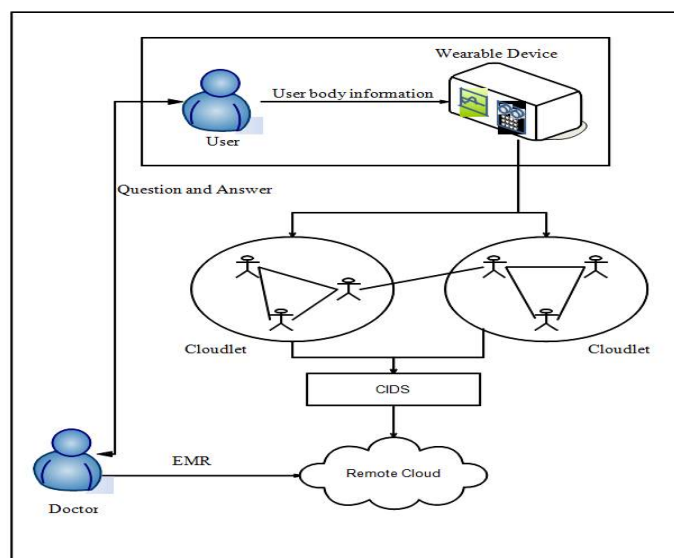
Fig 1. Architecture Diagram
