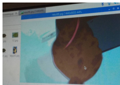
Figure 5.1: Segmentation image
