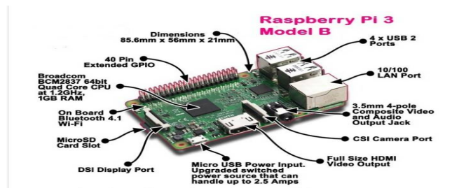
Figure.4.1.Raspberry pi
