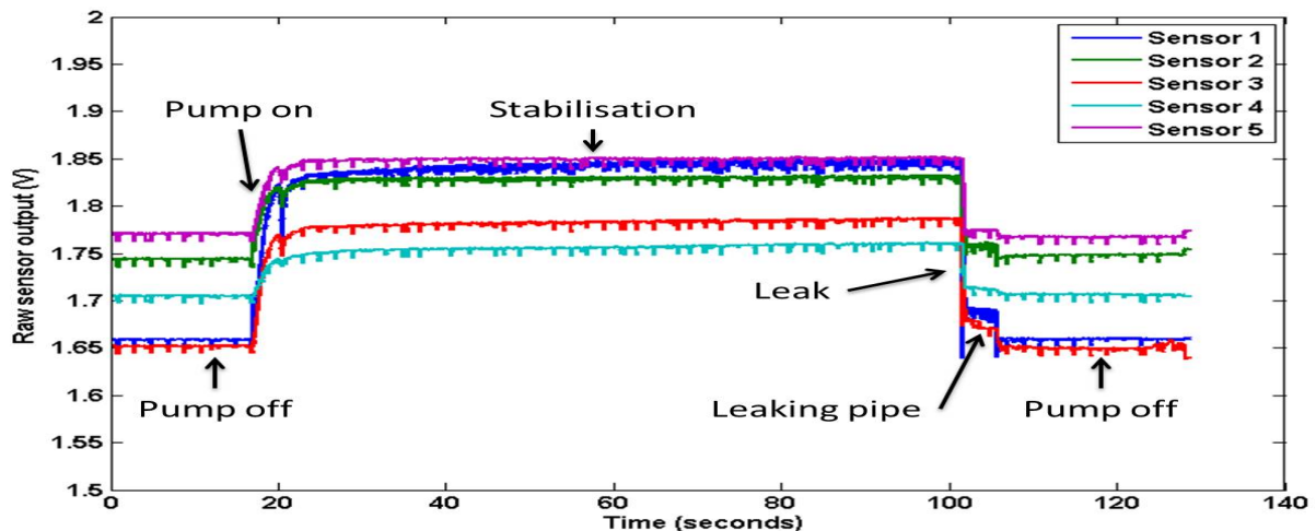
Figure: 6. Raw sensor output of laboratory experiment illustrating the pressure profiles for the five FSR sensors.
