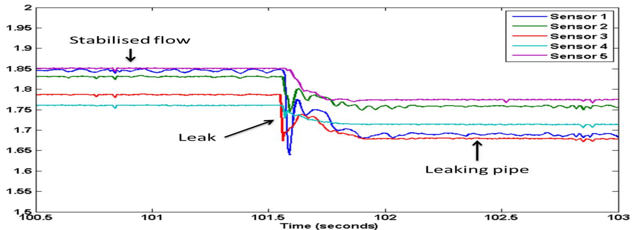
Figure 7. Pressure drop measured by the five FSR sensors due to the occurrence of the leak.
