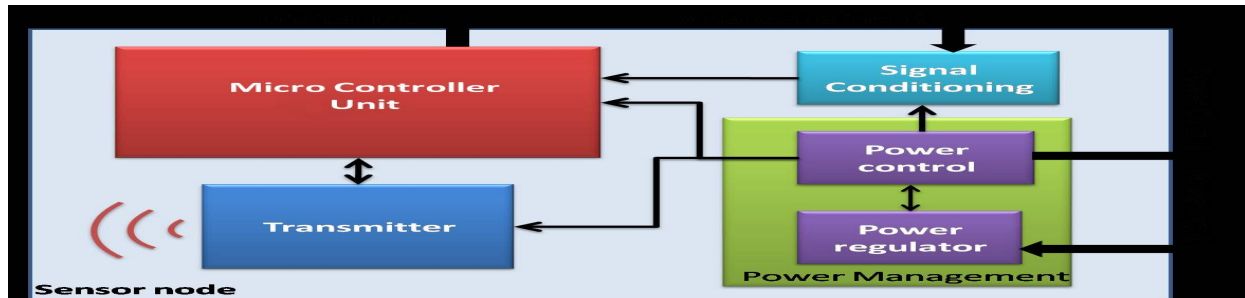
Figure 2. Schematic of the sensor node and its components.
