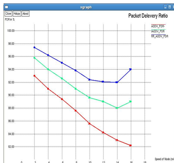
Fig. 6.4 Packet Delivery Ratio
