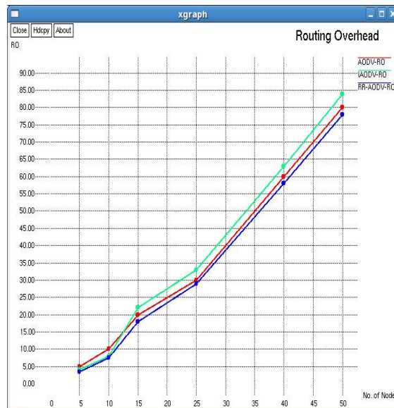
Fig. 6.2 Routing Overhead
