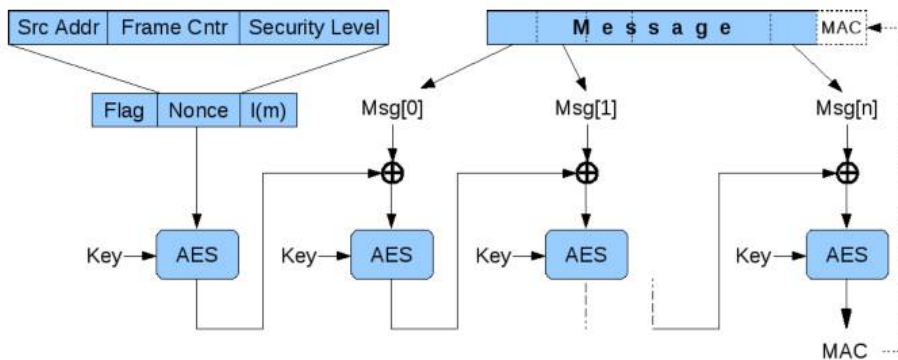
Figure 1. Authentication of a message according to CCM with AES
