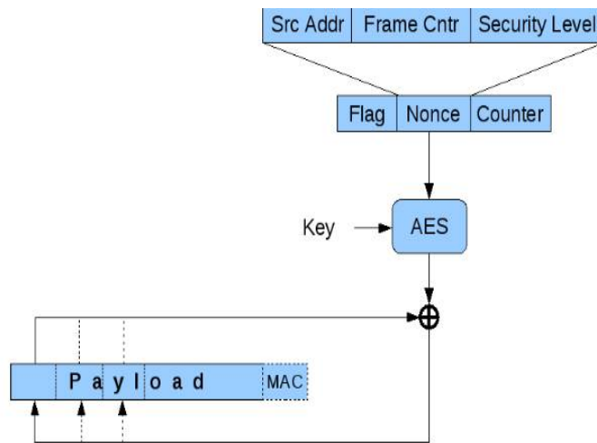
Figure 2. Encryption of a message according to CCM with AES
