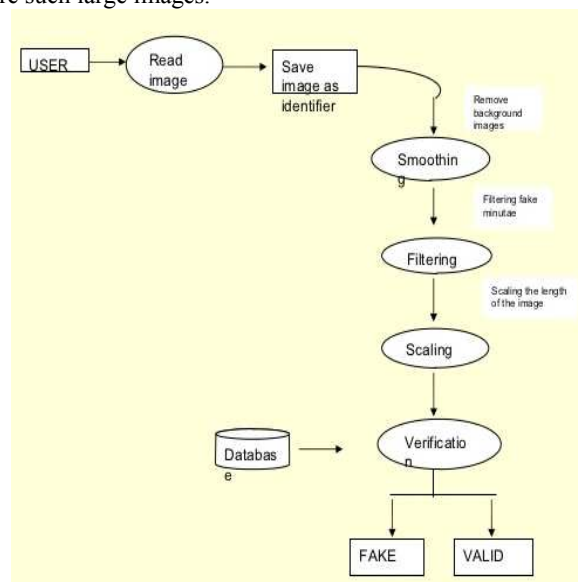
Fig.2 Proposed System Flow Diagram
