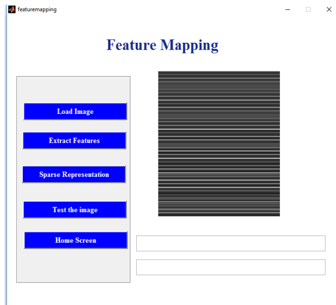
Fig.8 Feature Mapping
