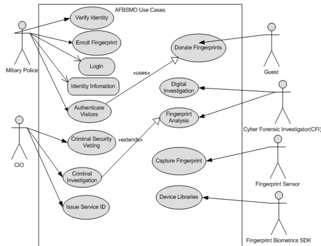
Fig.3 Proposed System Usecase Diagram
