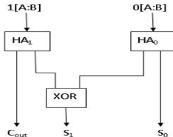
Figure 6: A Proposed 2 bit KS Adder
