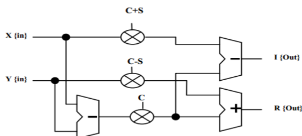
Figure 4: Implementation of complex multiplication
