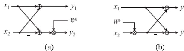
Figure 1: (a) DIF FFT butterfly (b) DIT FFT butterfly
