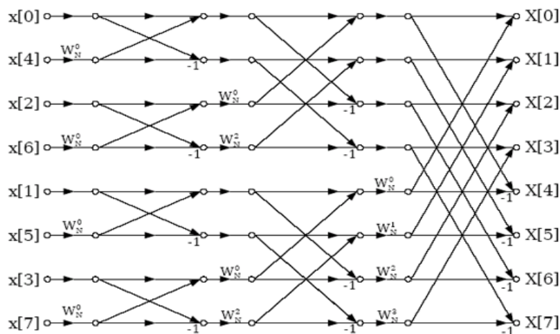
Figure 2: Radix-2 Decimation in Time Domain FFT Algorithm
