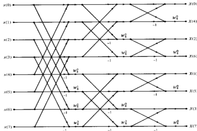
Figure 3: Radix-2 Decimation in Frequency Domain FFT Algorithm
