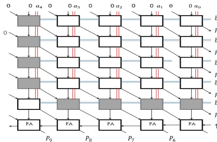
Figure 5: Signed Multiplier
