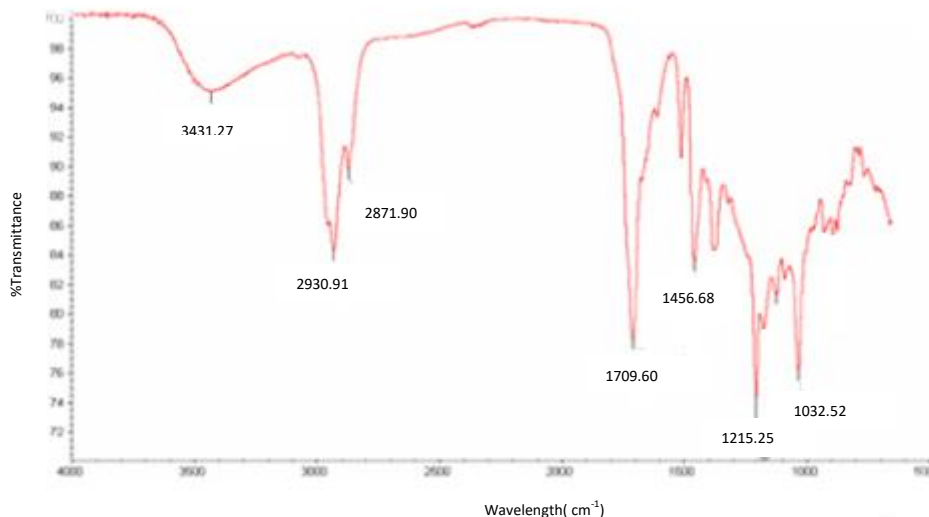
Figure 2: FT-IR spectrum of Acorus Calamus
