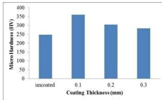
Fig. 1. Effect of coating thickness on Micro Hardness Wear test
