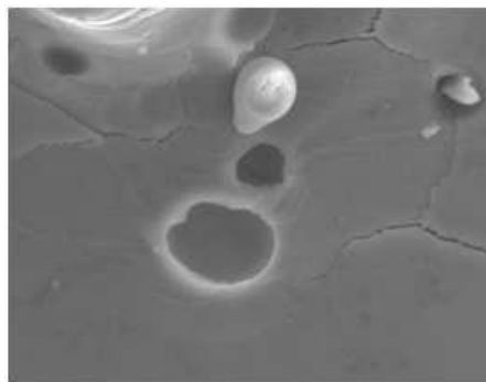
Fig. 6 Field Emission SEM images of 0.3 mm Air plasma sprayed coating, on the scale of 10 \mu m.
