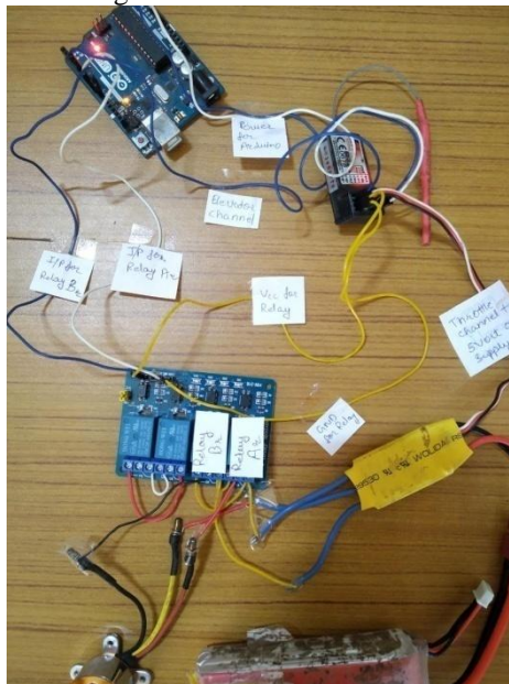
Fig. 3 Setup for the project
