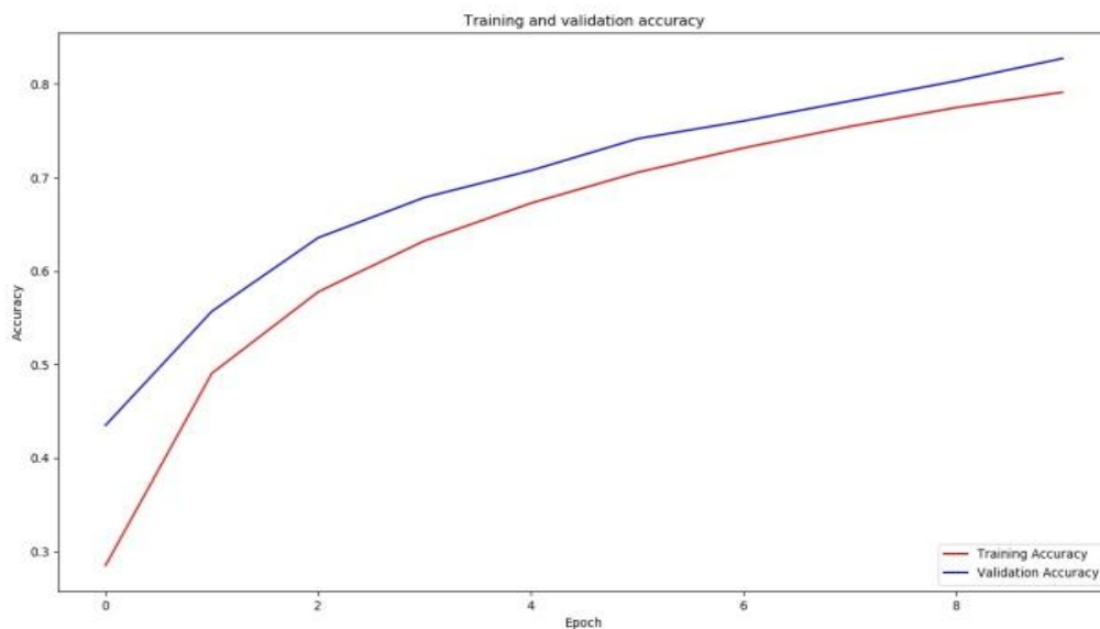
Fig:4 Training And Validation Accuracy
