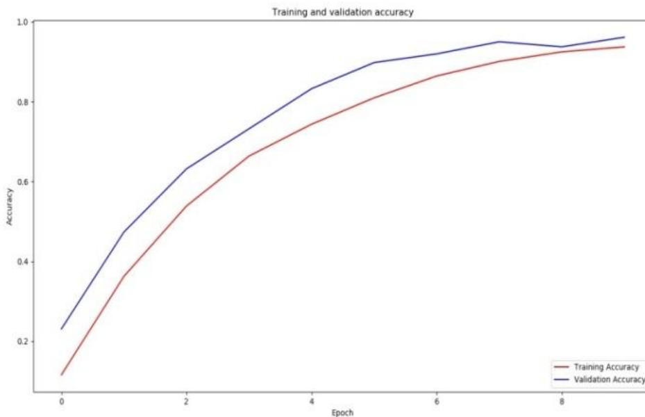
Fig:2 Training And Validation Accuracy
