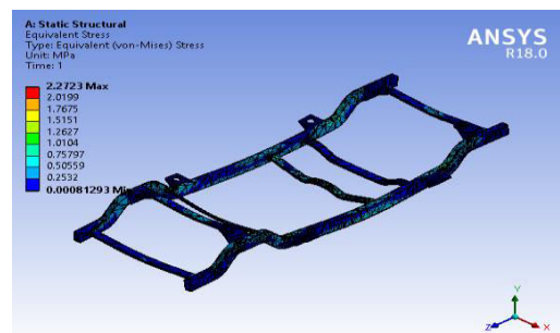
Fig 5. Von-Mises Stresses in Glass Fibre Chassis
