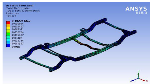
Fig. 4 Deformation in GF Chassis
