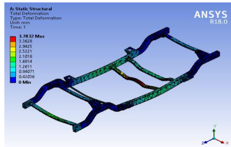
Fig 2. Deformation in Steel Chassis
