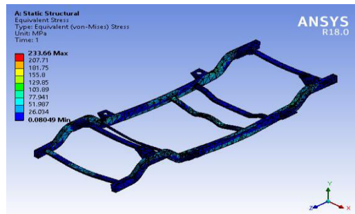
Fig.3 : Von-Mises Stresses in Steel chassis
