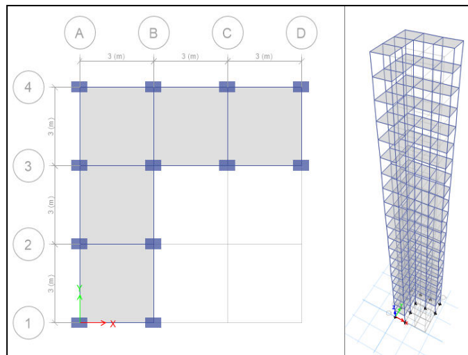
Fig.2 Plan and 3D view of Model 2
