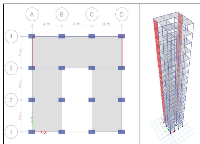
Fig.5 Plan and 3D view of Model 5
