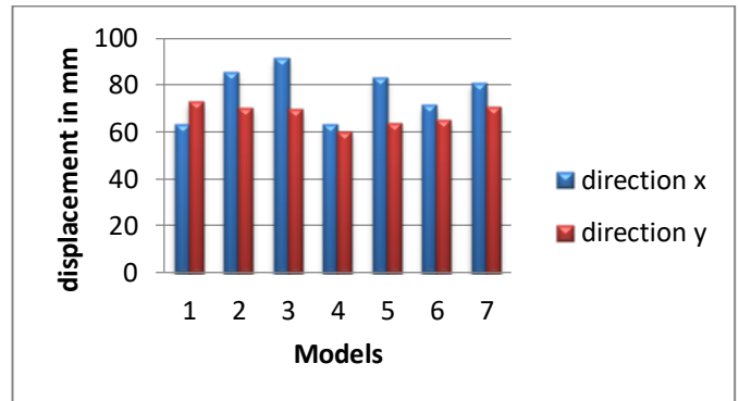
Fig.8 Maximum storey displacement
