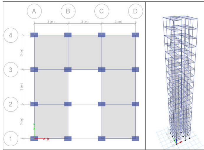
Fig.3 Plan and 3D view of Model 3
