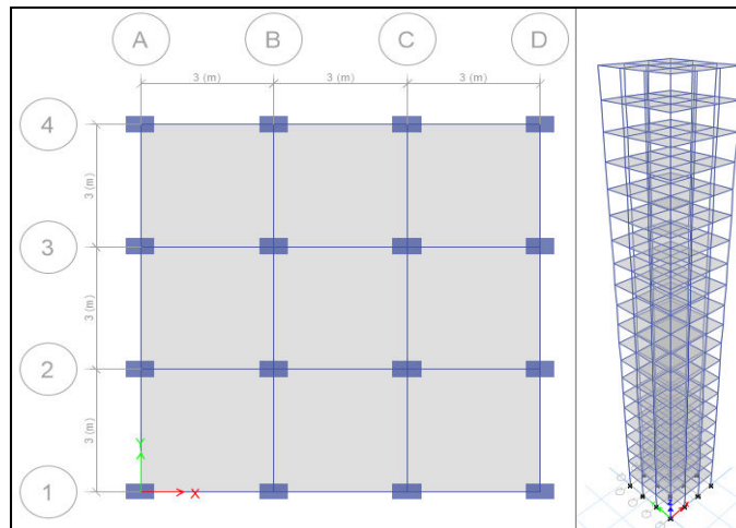
fig 1. Plan and 3D view of Model 1
