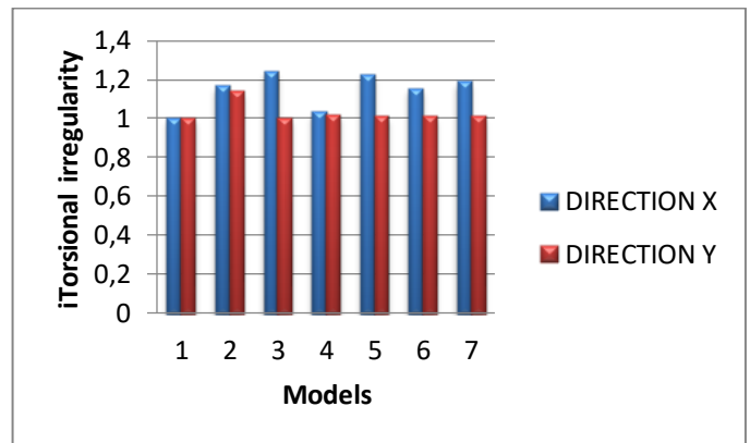
Fig. 11 TORSIONAL IRREGULARITY in X and Y direction
