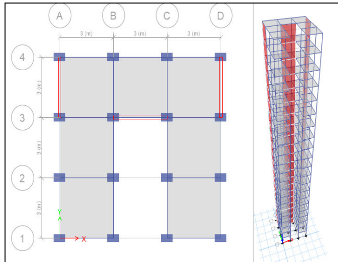
Fig.6 Plan and 3D view of Model 6
