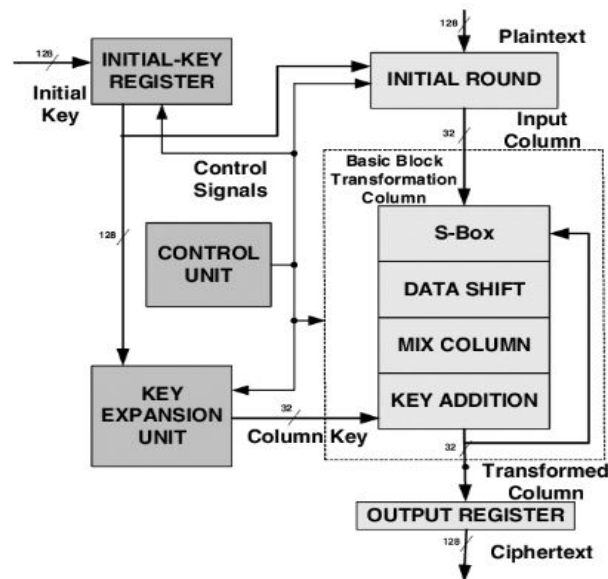
Figure 1: AES block diagram
