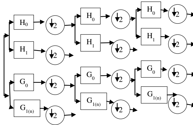
Fig. 1. Block diagram for DTCWT
