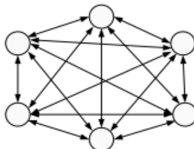
Fig.3 A gbest
