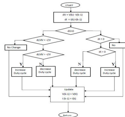
Fig 5 :Flow chart for Incremental Conductance
