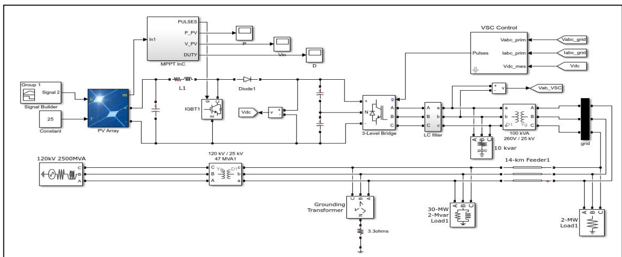
Fig17 : Simulink model of a 100 KW solar panel connected to a grid
