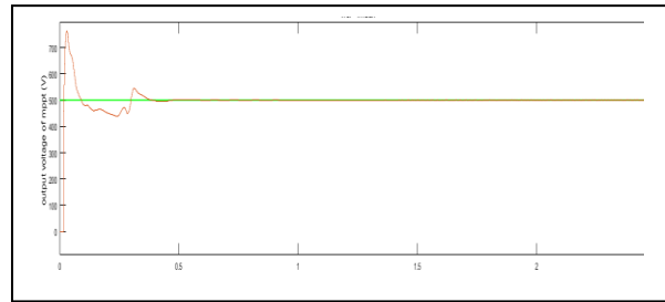
Fig 21: Boost Output Voltage
