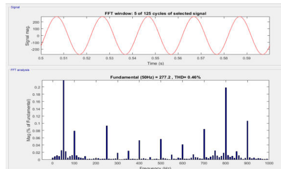
Fig12 : harmonic on output voltage with Filter
