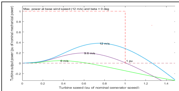
Fig 15: Wind Turbine power Curve ( \beta = 15 degree)
