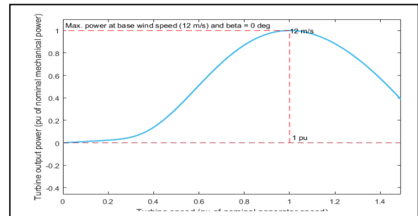
Fig 16: Wind Turbine Power Curve ( \beta = 0 degree)
