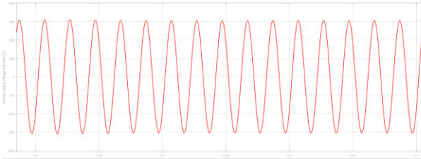
Fig9: Inverter output voltage with filter
