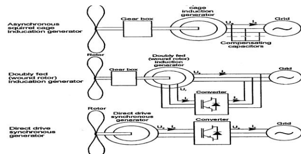
Fig 14 : Frequently occurring wind turbine type
