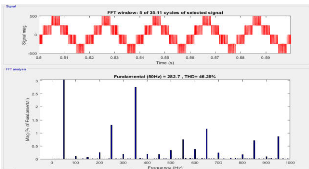
Fig11 : Plot of harmonic on output voltage without Filter
