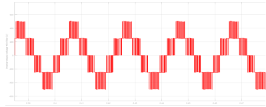
Fig10 : Inverter output voltage without filter
