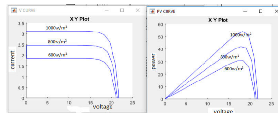
Fig 3: IV & PV Characteristics of PV array
