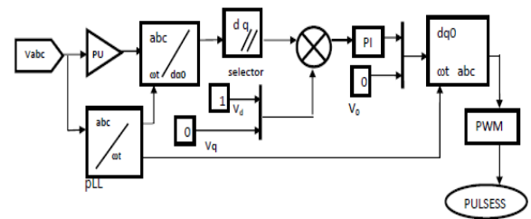
Fig13 : Control Topology of Voltage Control
