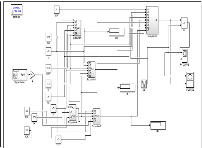
Fig1: Simulink model of PV panel with varying irradiance
