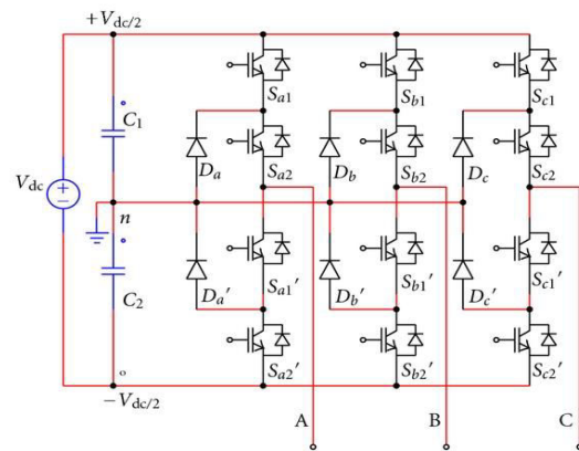
Fig 8: 3 level IGBT inverter
