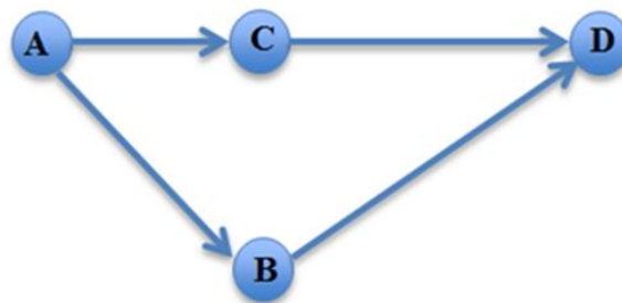
Fig. 1. Social Network.
