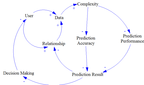
Fig. 2. Link Prediction Causal Loop.
