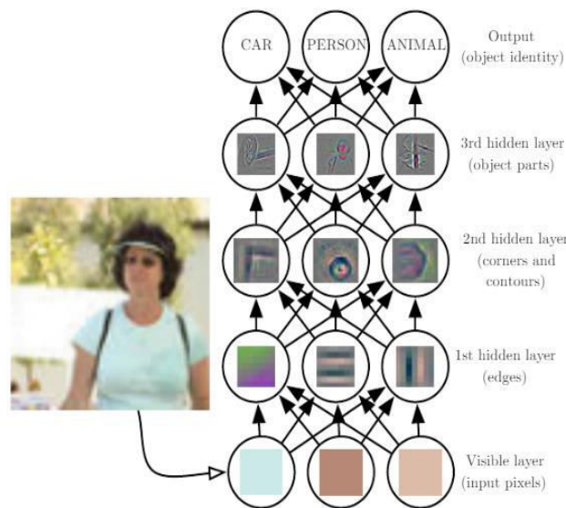
Fig. 2: Neural Network
