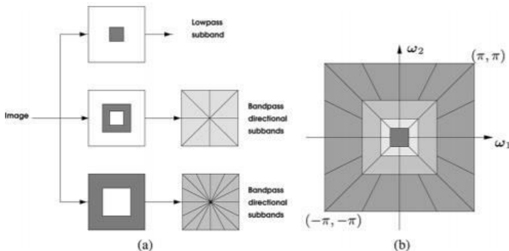
Fig. 1: Nonsubsampled contourlet transform. (a) NSFB structure that implements the NSCT. (b) Idealized frequency partitioning obtained with the proposed structure.
