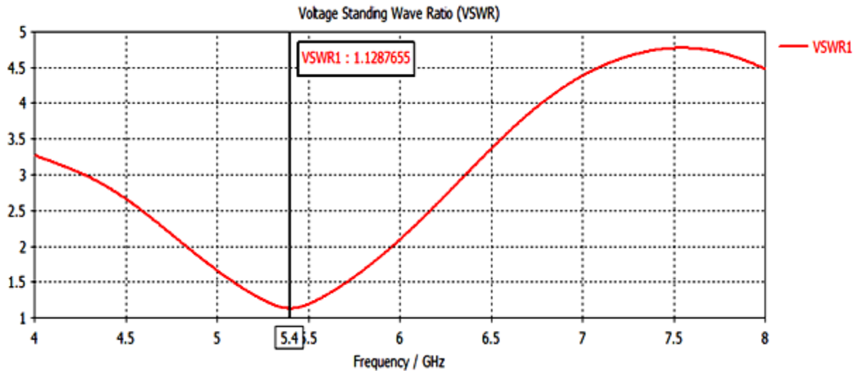
Figure 7: VSWR
