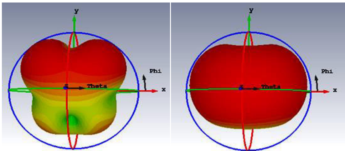
Figure 8: 3D Radiation pattern of proposed antenna
