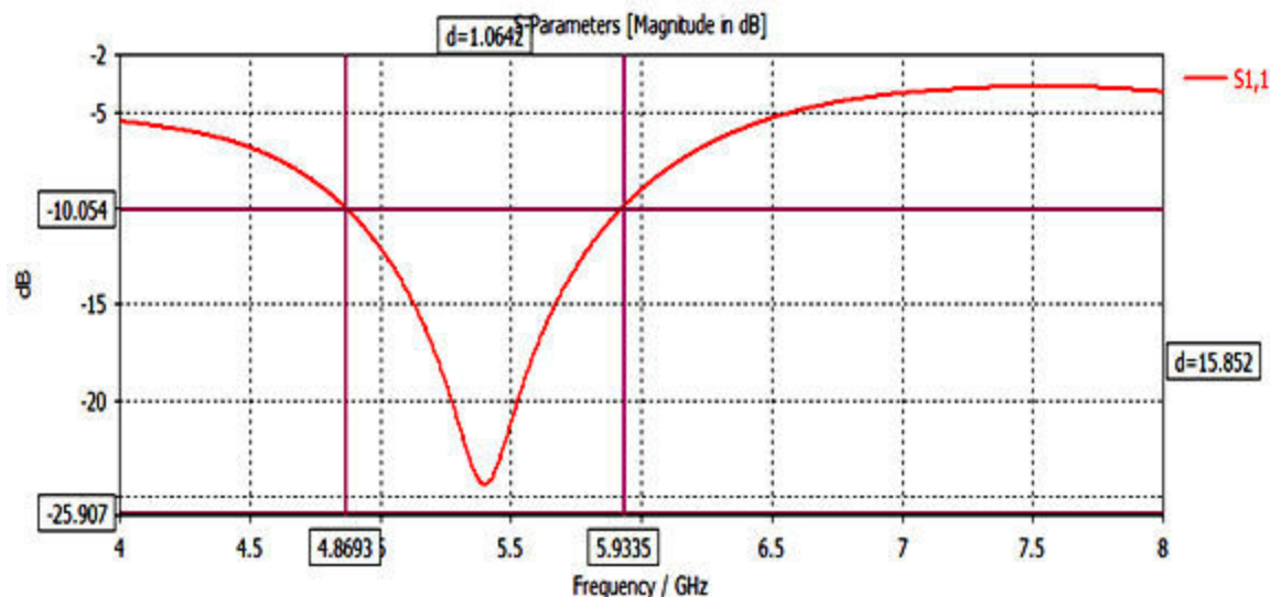
Figure 6: Bandwidth calculation of band
