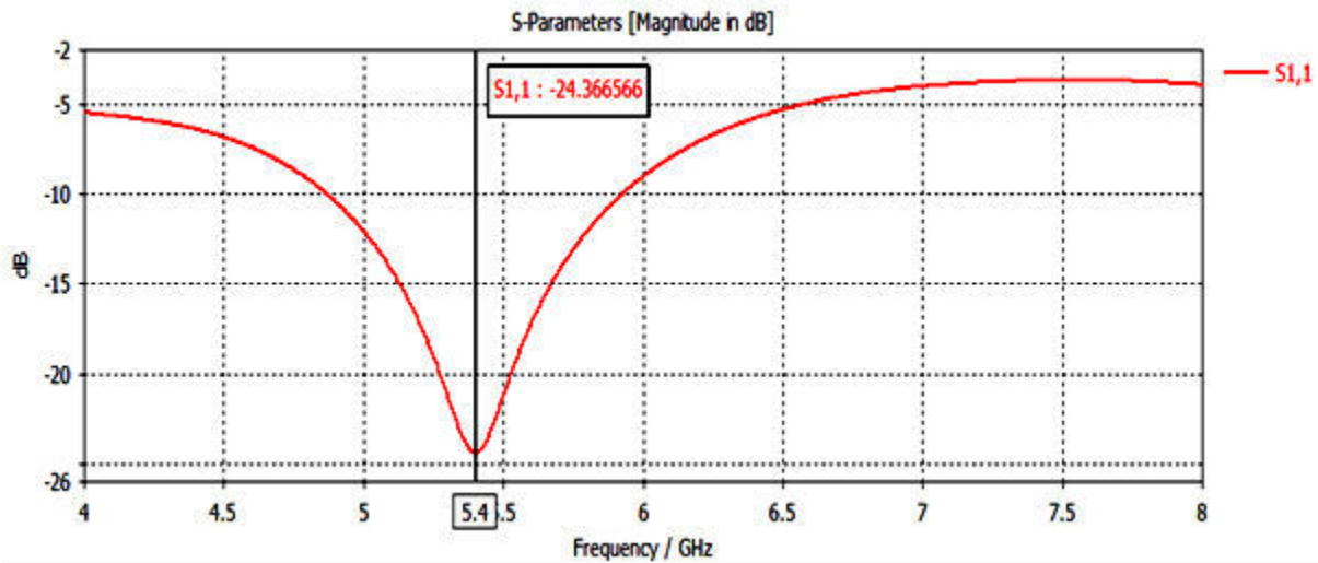
Figure 5: Return loss of band
