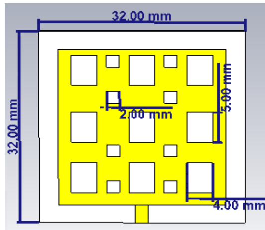
Figure 3: Dimension of proposed antenna
