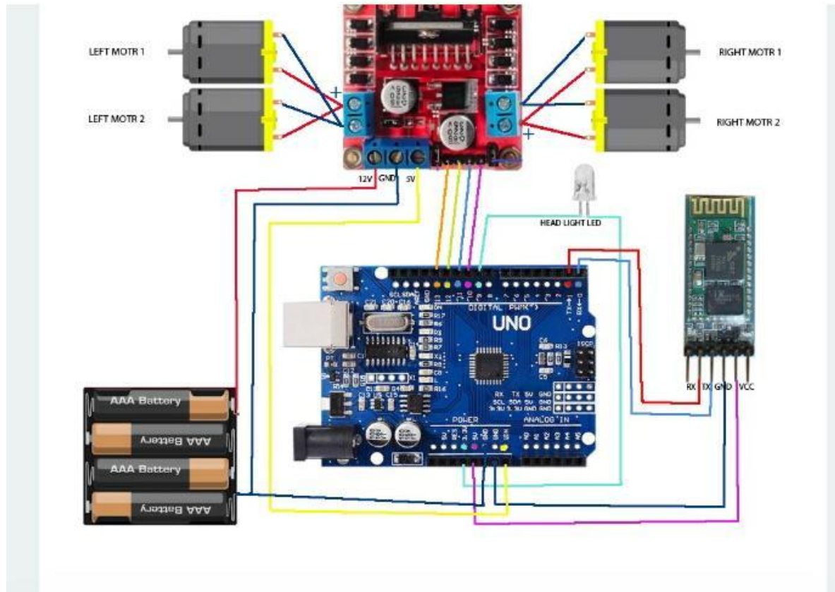
Figure 1 block diagram of purpose system
