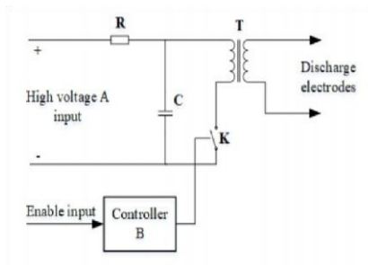
Fig6:Shock generator
