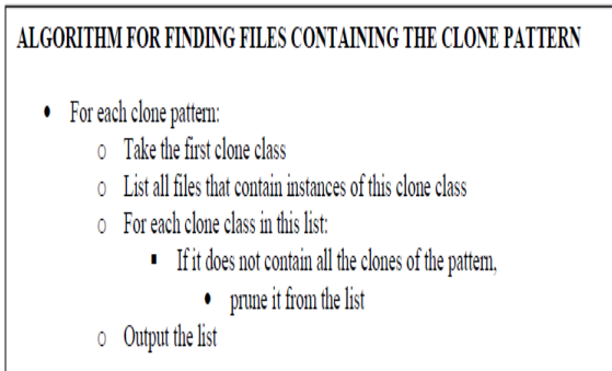
Fig 8 – Algorithm for finding Simple Clone pattern
