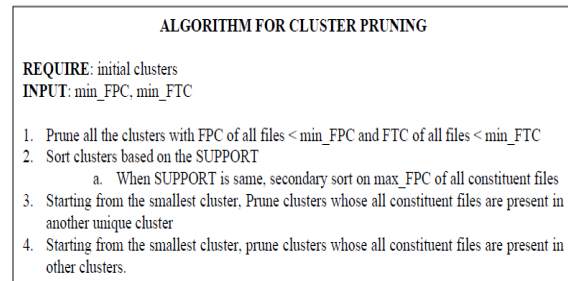
Fig 9 - Algorithm for cluster pruning
