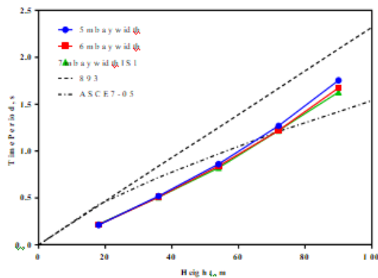
Figure 13. Variation of fundamental time period with bay width for Type - R building.
