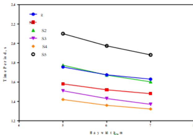
Figure 23. Variation of fundamental time period with bay width for 30-storey setback buildings
