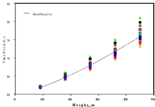
Figure 24. Regression analysis for Fundamental time period for models
