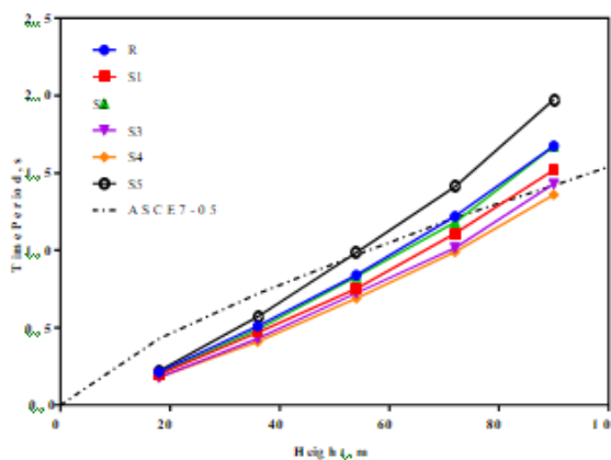
Figure 10. Comparison of fundamental period versus height of setback buildings of 6m bay width with that obtained from ASCE 7-05
