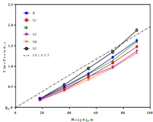
Figure 11. Comparison of fundamental period versus height of setback buildings of 7m bay width with that obtained from IS 1893
