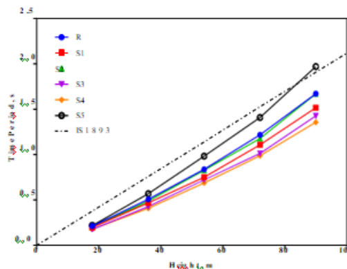
Figure 9. Comparison of fundamental period versus height of setback buildings of 6m bay width with that obtained from IS 1893
