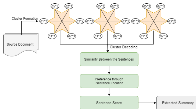
Fig -1: Flow-Chart of Cluster Based Algorithm
