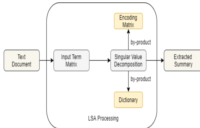
Fig -4: System Architecture – Latent Semantic Analysis
