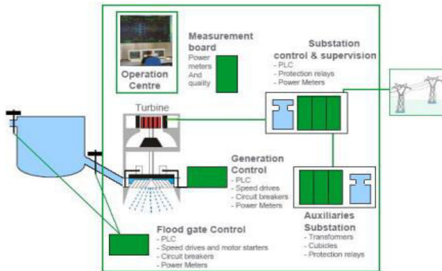
Figure 1: Automation system for SHP station [4]
