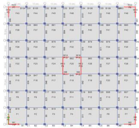
Figure 3(b): Model B
