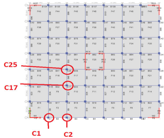
Figure 4(b): Column removal cases for Model B
