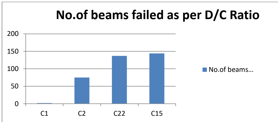
Figure 5(a): No. of beams failed as per D/C Ratio
