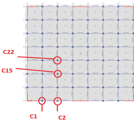
Figure 4(a): Column removal cases for Model A
