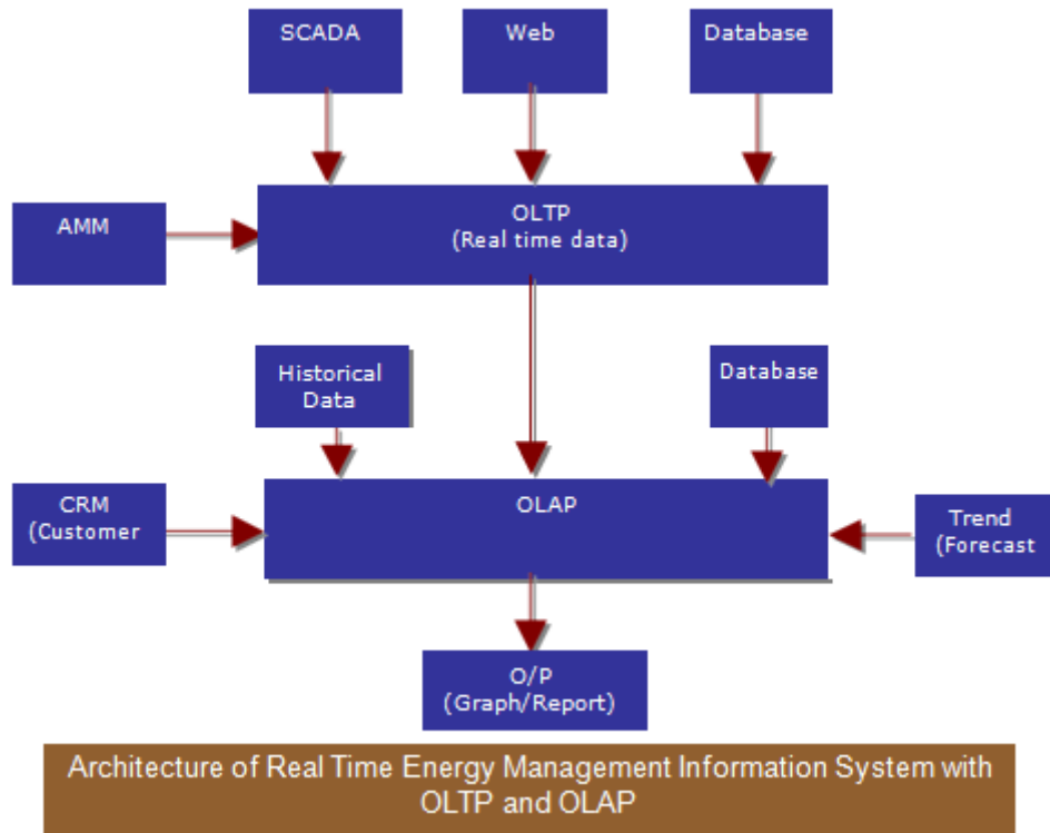
Fig 1 Block diagram of Real Time Energy Management Information System with OLTP and OLAP. Architecture of above interfaces is discussed below
