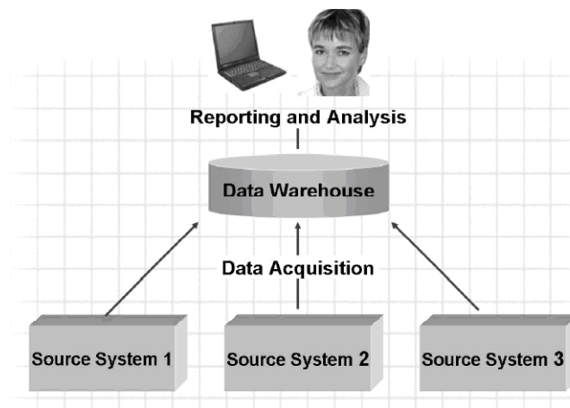
Fig 3 Heterogeneous Source System Environment
