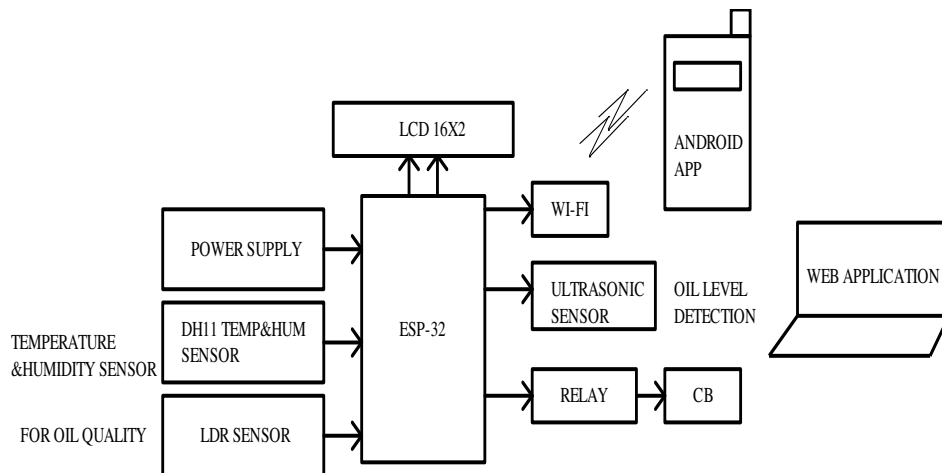
Fig 2.1 Block Diagram
