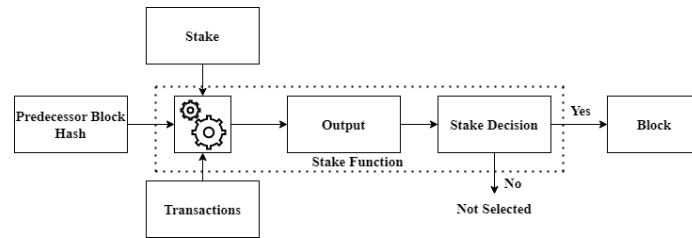
Fig. 3. Working of Proof-of-Stake
