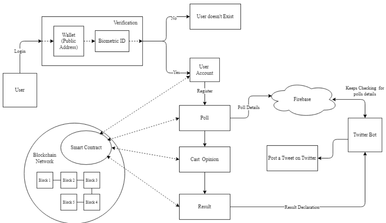
Fig. 2. System architecture
