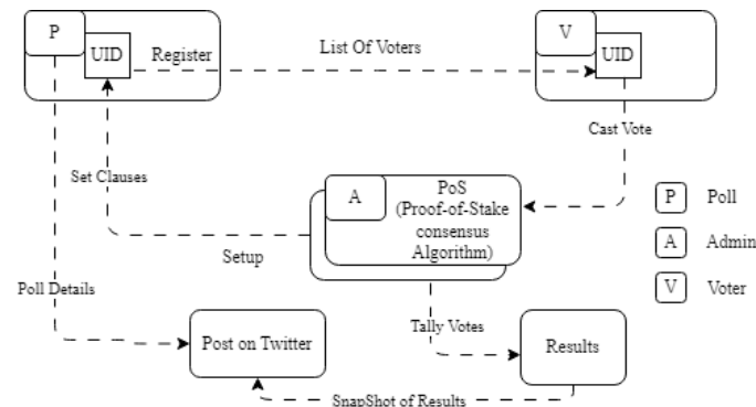
Fig. 4. System Overview
