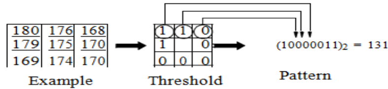
Fig. 1. The basic LBP operator.
