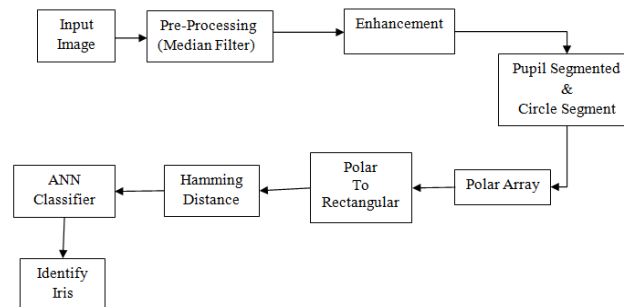
Fig.3: Existing Block Diagram
