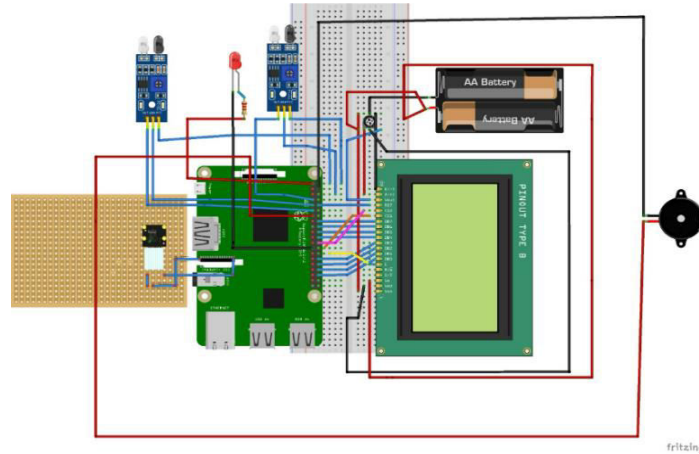
Planned Circuit diagram.
