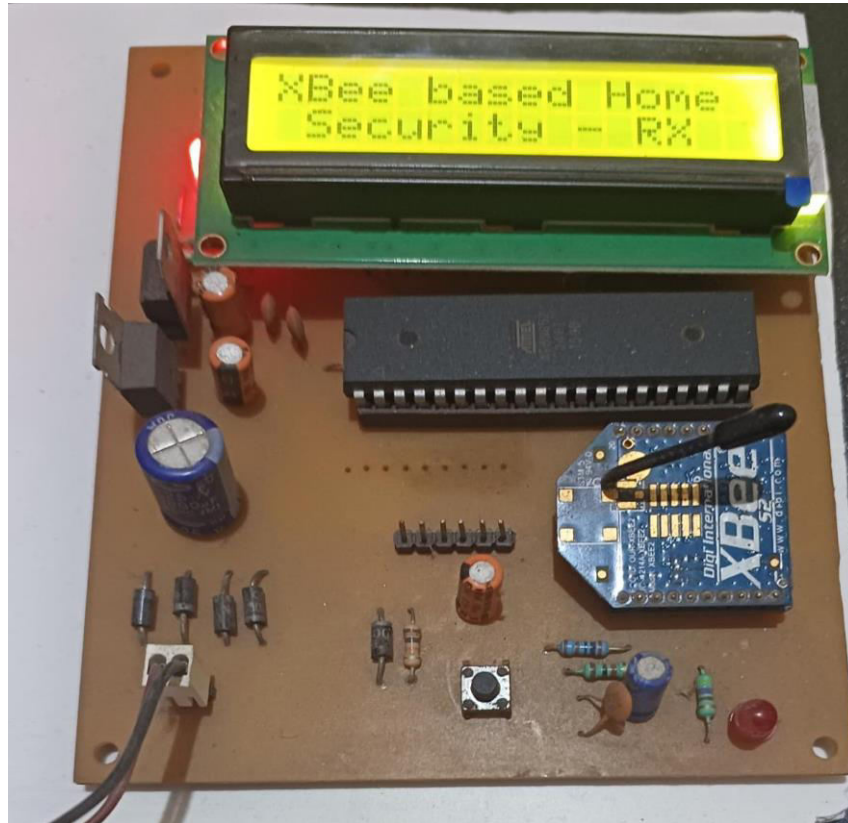
Fig.1 Circuit of the Project.
