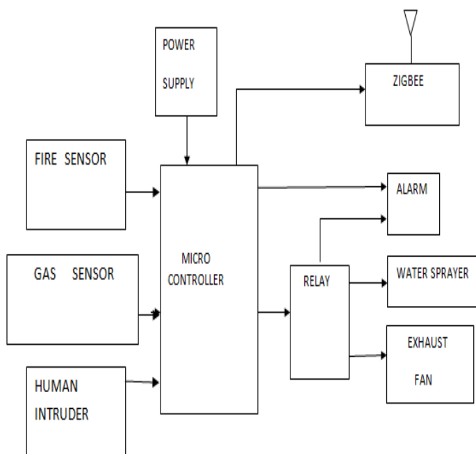
Fig.3.Block Diagram of System.
