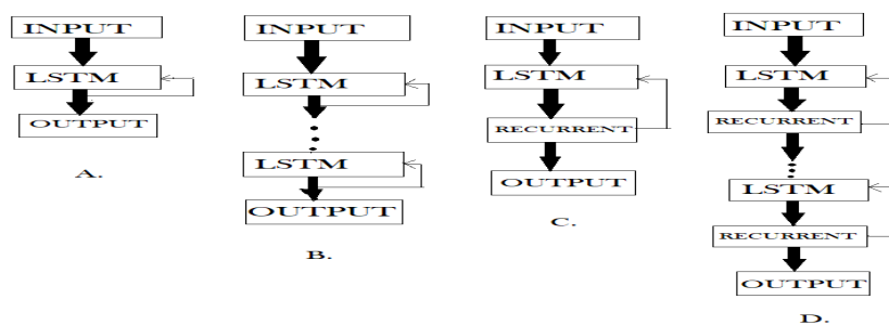
LSTM Classification
