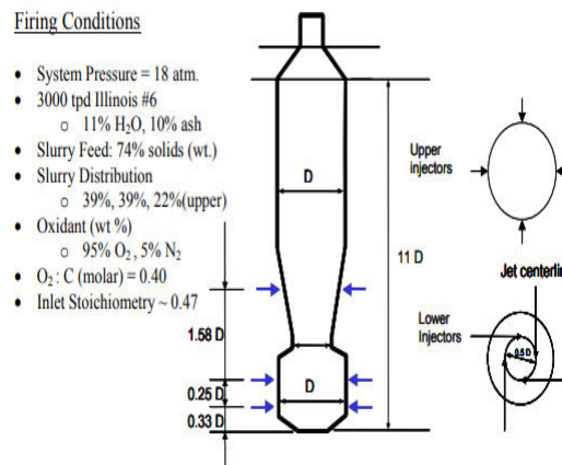
Figure-3: Schematic of two-stage up-flow configuration and summary of process condition
