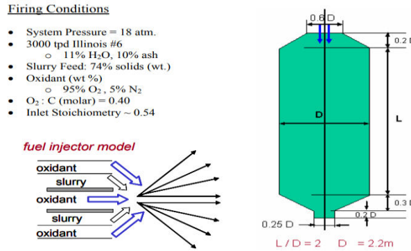
Figure-2: Schematic of one-stage, slurry-feed, downflow gasifier and process conditions.
