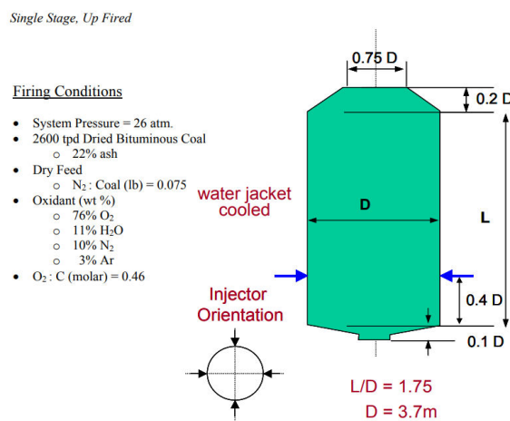
Figure-1: Schematic of single-stage, up-fired gasifier and summary of process conditions.
