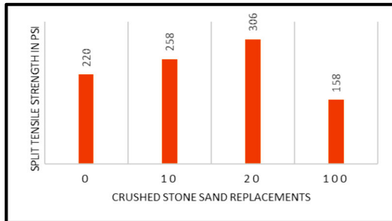
Fig 10: Split tensile strength values at 7 days curing period.
