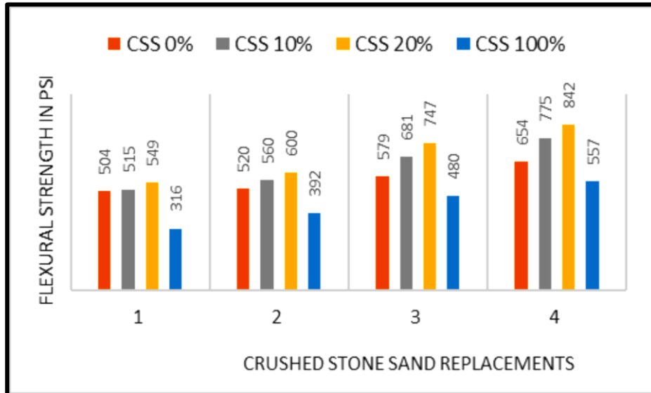
Fig 9: Flexural strength values of concrete mixes modified with different substitutions of crushed stone sand replacements levels for 7, 14, 28 & 56.
