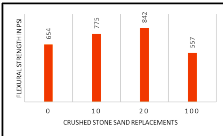
Fig 8: Flexural strength values at 56 days curing period.
