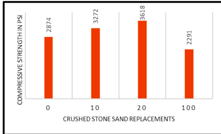
Fig 3: Compressive strength values at 28 days curing period.
