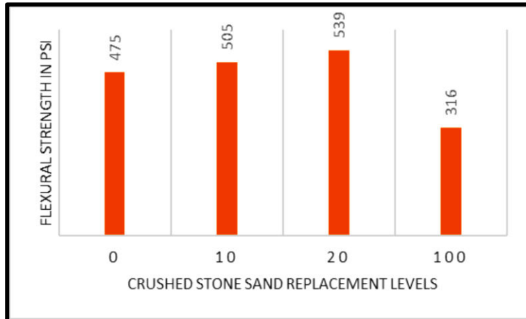
Fig 6: Flexural strength values at 7 days curing period.
