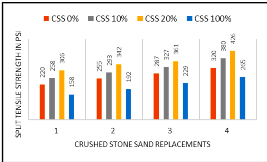
Fig 13: Split tensile strength values of concrete mixes modified with different substitutions of crushed stone sand replacements levels for 7, 14, 28 & 56.
