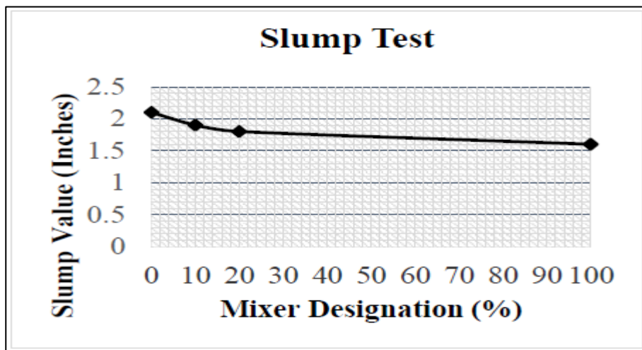
Fig 1. Slump values for varying crushed stone percentages
