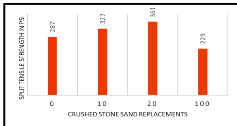
Fig 11: Split tensile strength values at 28 days curing period.
