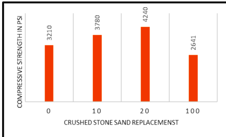
Fig 4: Compressive strength values at 56 days curing period.
