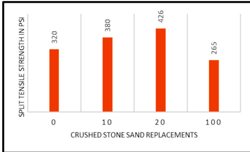
Fig 12: Split tensile strength values at 56 days curing period.
