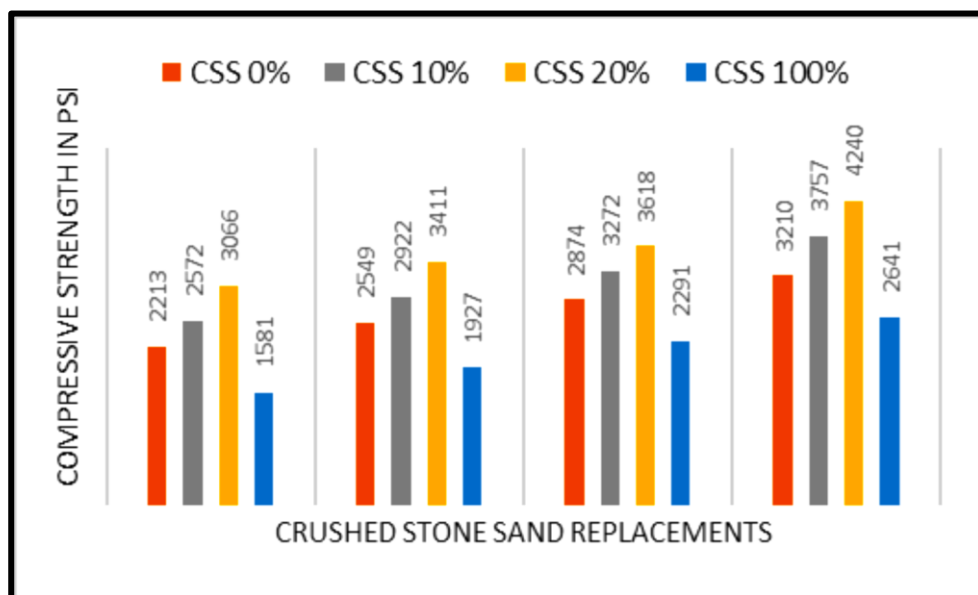
Fig 5: Compressive strength values of concrete mixes modified with different substitutions of crushed stone sand replacements levels for 7, 14, 28 & 56.
