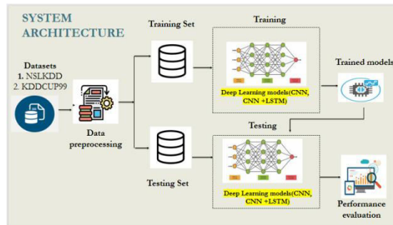
Fig 1 Proposed Architecture
