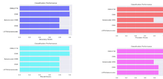
Fig 12 Comparison Graphs of NSL - KDD
