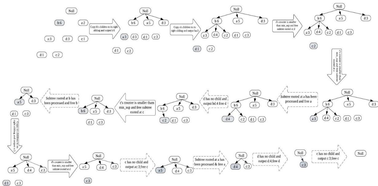
Figure 2. DPT Runtime
