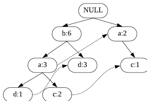
Figure 1. Prefix Tree
