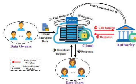
Fig. 1 Cloud Architecture
